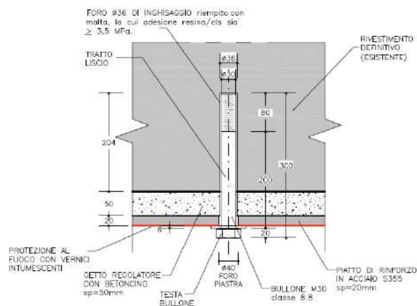
Figure 10. Intervention with steel plates: detail
