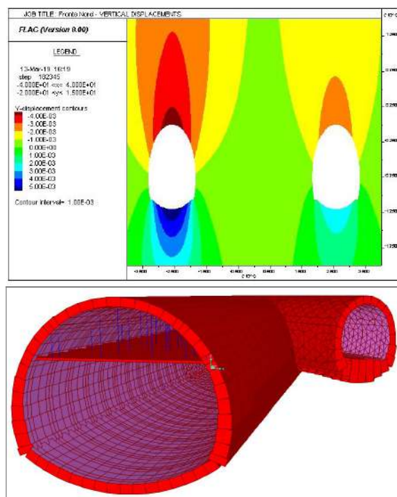
Figure 7. Examples of 2D-3D FEM numerical models
