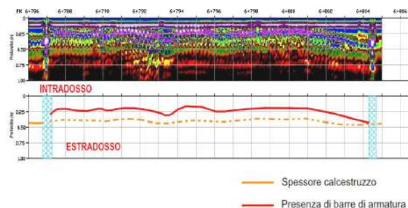
Figure 1. Georadar investigation
