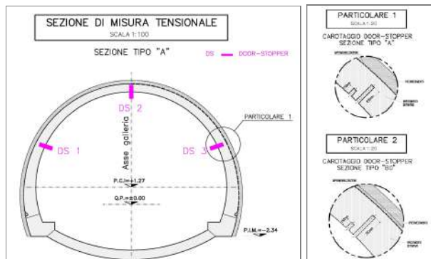
Figure 3. Doorstopper tests' location
