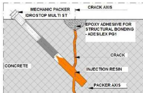
Figure 8. Cracks' sealing procedure
