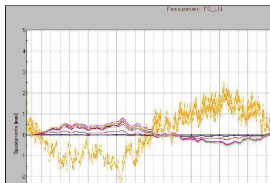
Figure 12. Variation of crack's opening vs temperature
