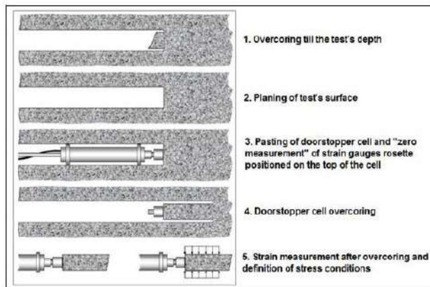
Figure 2. Doorstopper test
