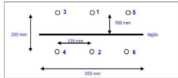
Figure 4. Flat-jack scheme
