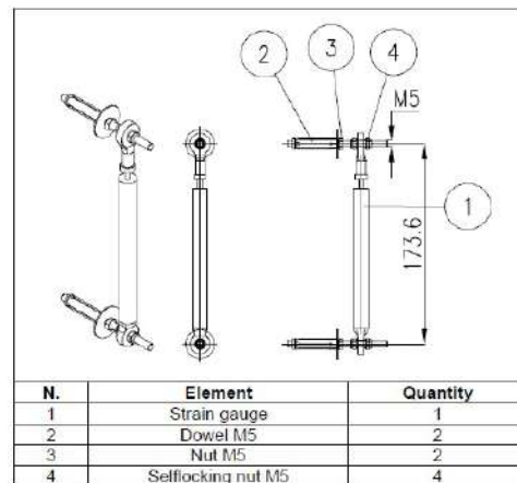
Figure 5. Electrical crack-meters
