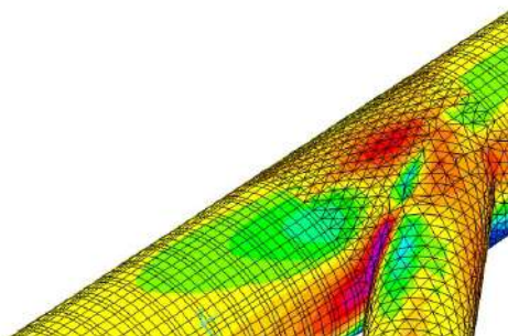
Figure 16. 3D FEM Model for local stresses' evaluation
