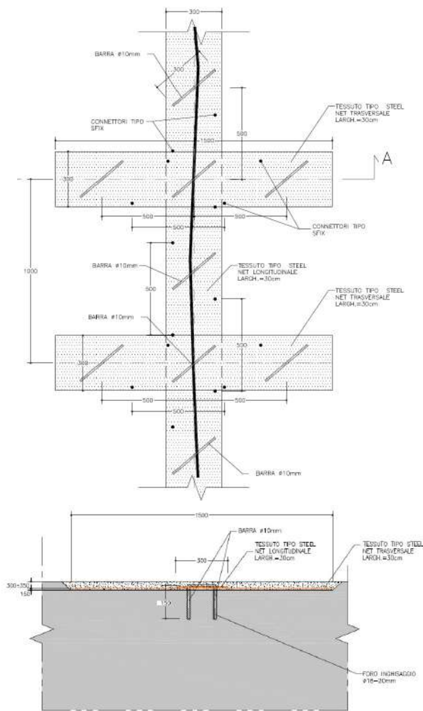
Figure 9. UHTTS steel net fabric intervention
